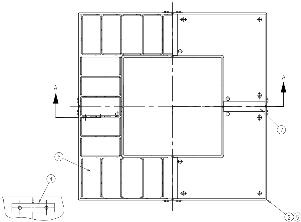
C矢視 (1:4)
